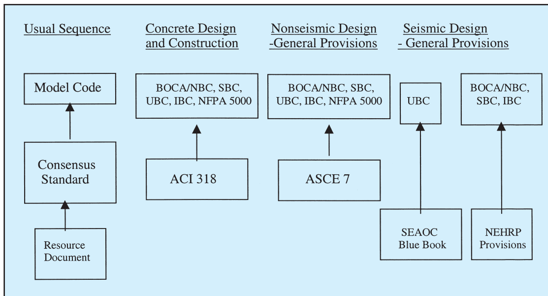
Fig. 2. Seismic design provisions and concrete design and construction provisions in various codes and standards.
